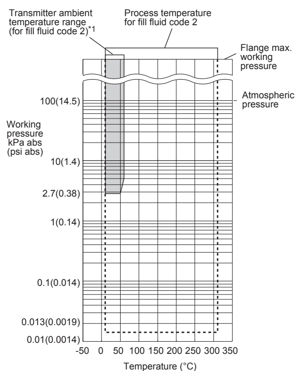
Figure 1-4. Working Pressure and Process Temperature (Fill fluid: silicone oil for high temp. and high vacuum use)
